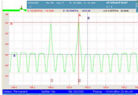
14 channel ROAD network, with 12 channels blocked and 2 channels passing
